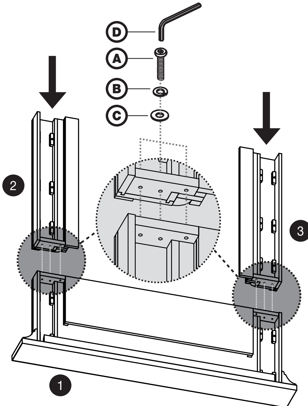
A | Bolt 1/4" x 64mm | x6
